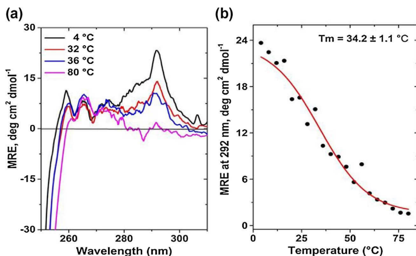
Fig. 7. Thermal stability of the tertiary structure of hisPS2. (a) Near-UV CD spectra of hisPS2 at 4 °C, 32 °C, 36 °C, and 80 °C. HisPS2 in SEC buffer was unfolded at an increasing temperature. Near-UV CD spectra recorded at different temperatures demonstrated a progressive loss of tertiary structure. (b) Thermal unfolding of hisPS2 tertiary structure monitored by CD signal at 292 nm. Solid line represents the Boltzmann fit.
